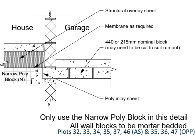
JF155 - Internal Loadbearing Wall (House / Garage)
