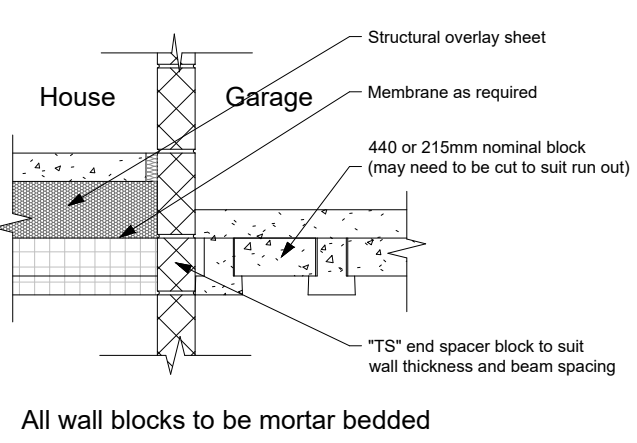
JF154 - Internal Loadbearing Wall (House / Garage)
